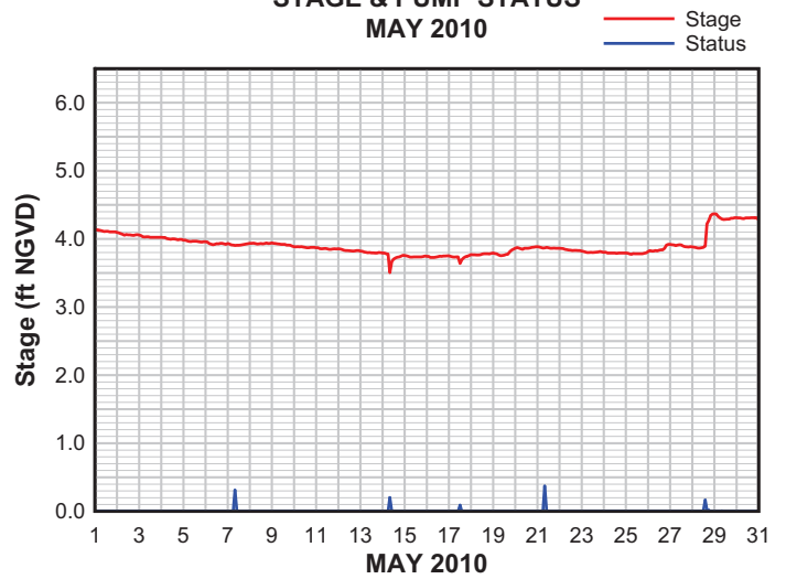
PUMP STATION 4 STAGE & PUMP STATUS MAY 2010
