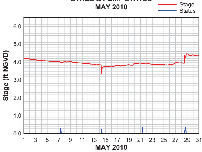
PUMP STATION 3 STAGE & PUMP STATUS MAY 2010
