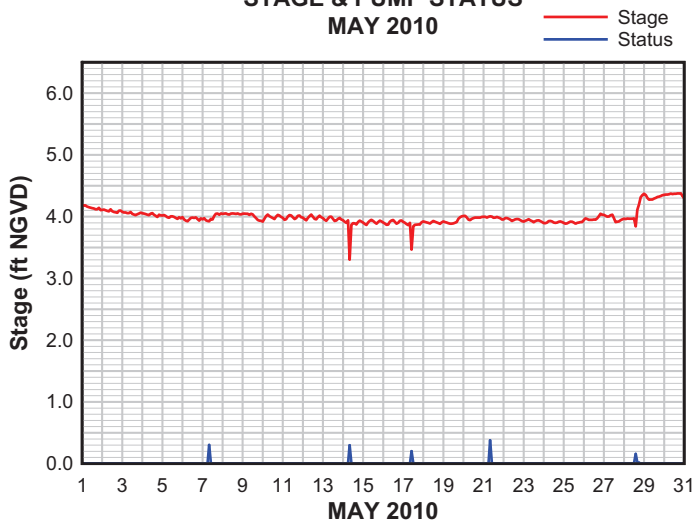
PUMP STATION 5 STAGE & PUMP STATUS MAY 2010
