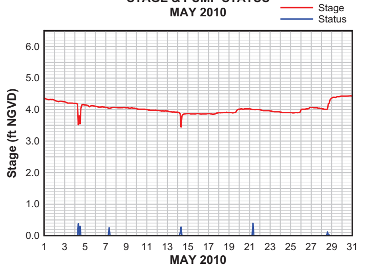
PUMP STATION 2 STAGE & PUMP STATUS MAY 2010
