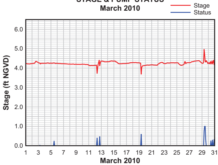
PUMP STATION 5 STAGE & PUMP STATUS March 2010
