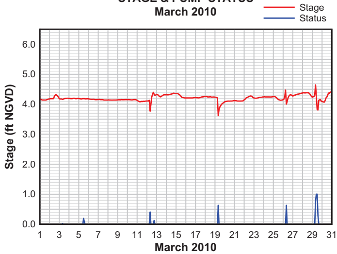
PUMP STATION 3 STAGE & PUMP STATUS March 2010
