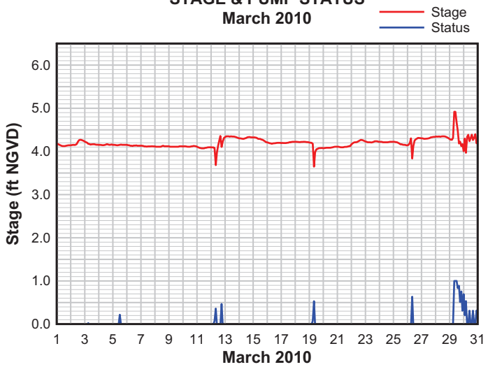
PUMP STATION 6 STAGE & PUMP STATUS March 2010
