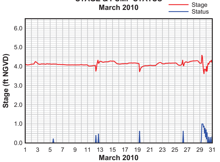
PUMP STATION 4 STAGE & PUMP STATUS March 2010
