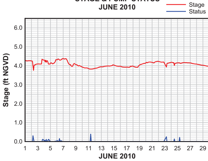
PUMP STATION 3 STAGE & PUMP STATUS JUNE 2010
