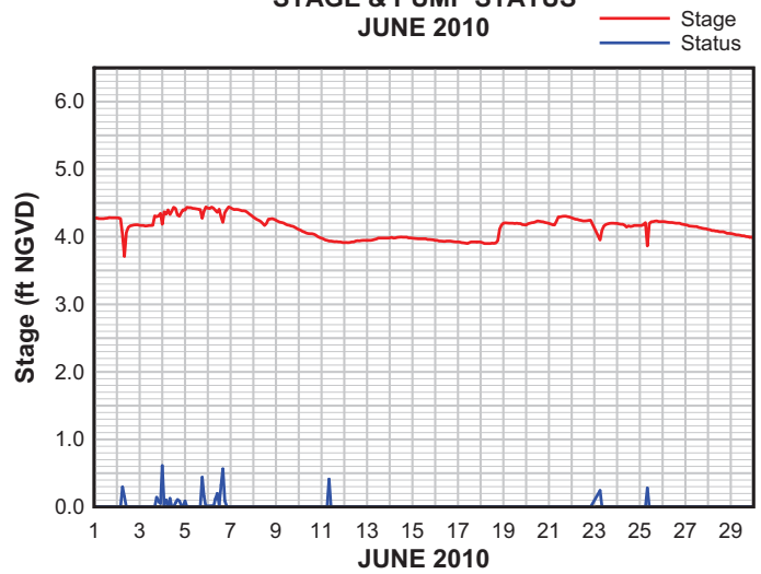
PUMP STATION 6 STAGE & PUMP STATUS JUNE 2010
