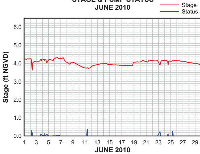
PUMP STATION 5 STAGE & PUMP STATUS JUNE 2010
