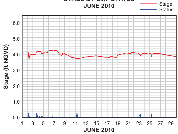
PUMP STATION 4 STAGE & PUMP STATUS JUNE 2010
