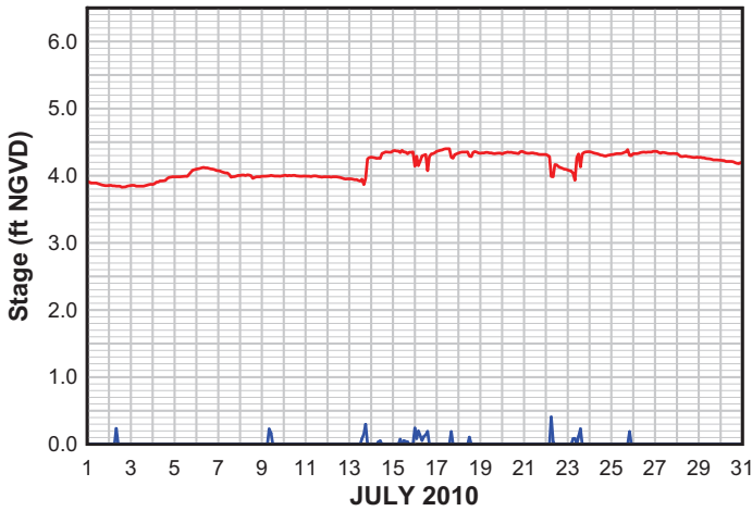
PUMP STATION 3 STAGE & PUMP STATUS JULY 2010
