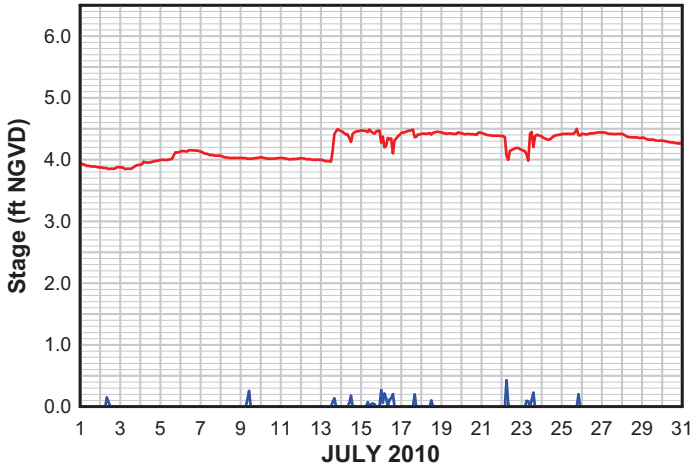
PUMP STATION 1 STAGE & PUMP STATUS JULY 2010
