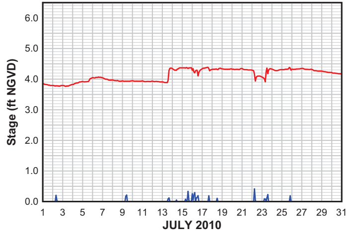
PUMP STATION 2 STAGE & PUMP STATUS JULY 2010
