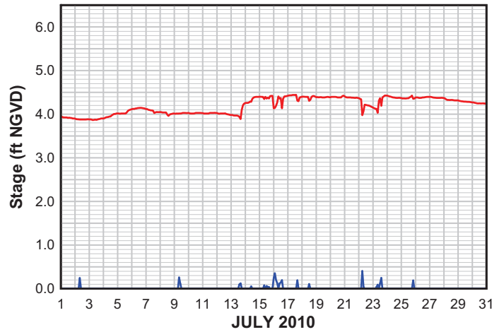
PUMP STATION 4 STAGE & PUMP STATUS JULY 2010
