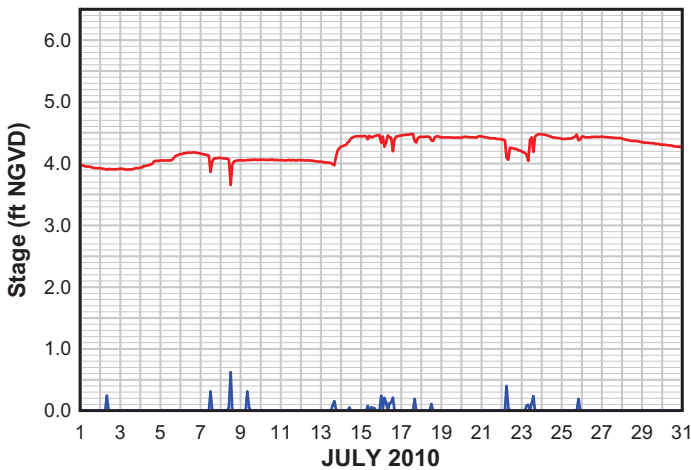
PUMP STATION 5 STAGE & PUMP STATUS JULY 2010
