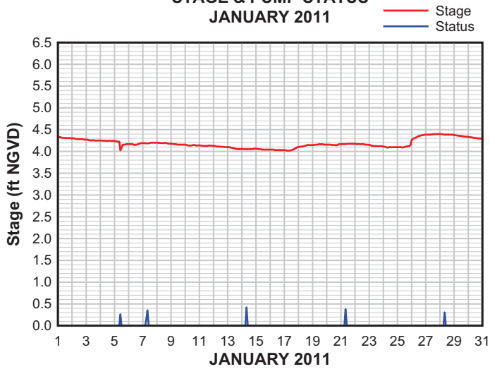
PUMP STATION 4 STAGE & PUMP STATUS JANUARY 2011
