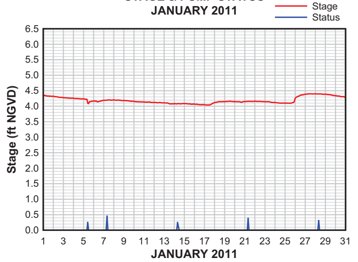
PUMP STATION 6 STAGE & PUMP STATUS JANUARY 2011
