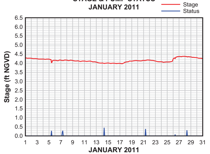
PUMP STATION 2 STAGE & PUMP STATUS JANUARY 2011
