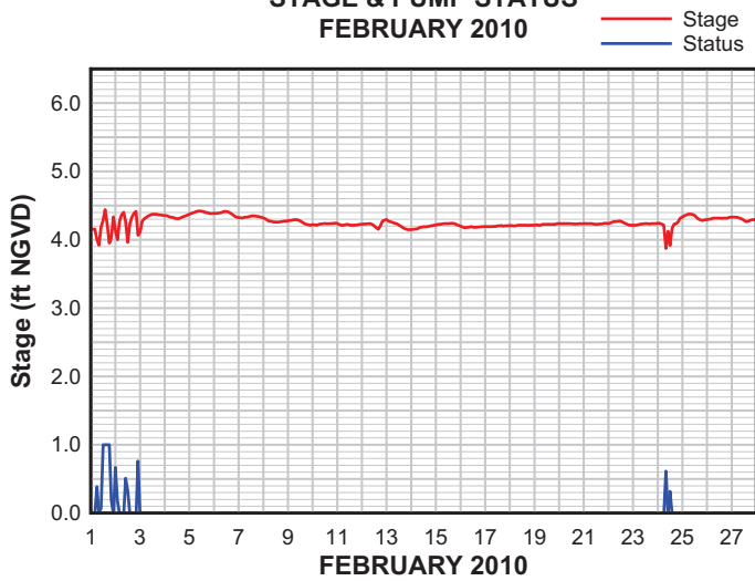
PUMP STATION 5 STAGE & PUMP STATUS FEBRUARY 2010
