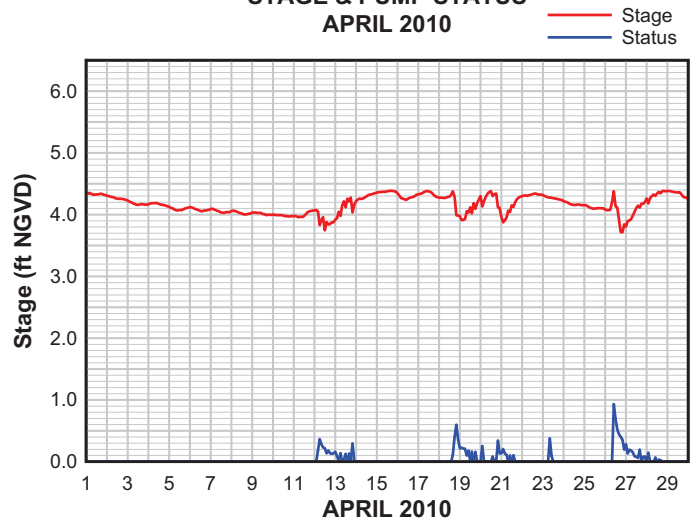
PUMP STATION 3 STAGE & PUMP STATUS APRIL 2010
