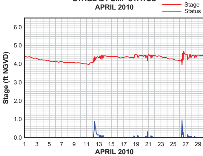
PUMP STATION 2 STAGE & PUMP STATUS APRIL 2010
