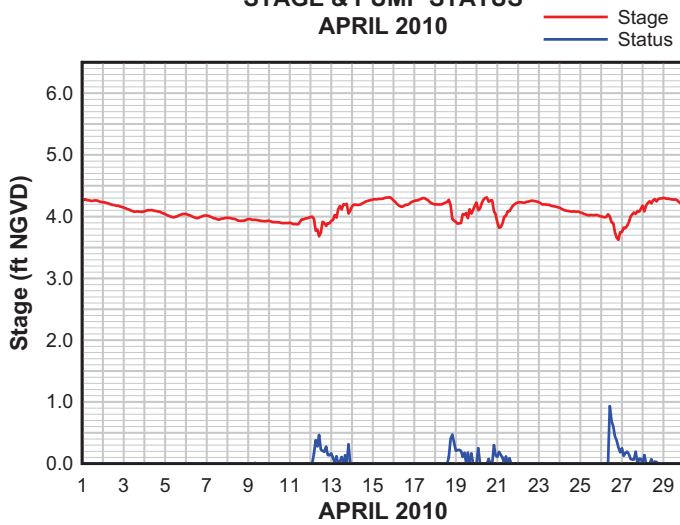
PUMP STATION 4 STAGE & PUMP STATUS APRIL 2010
