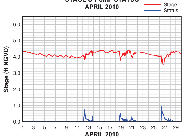
PUMP STATION 5 STAGE & PUMP STATUS APRIL 2010
